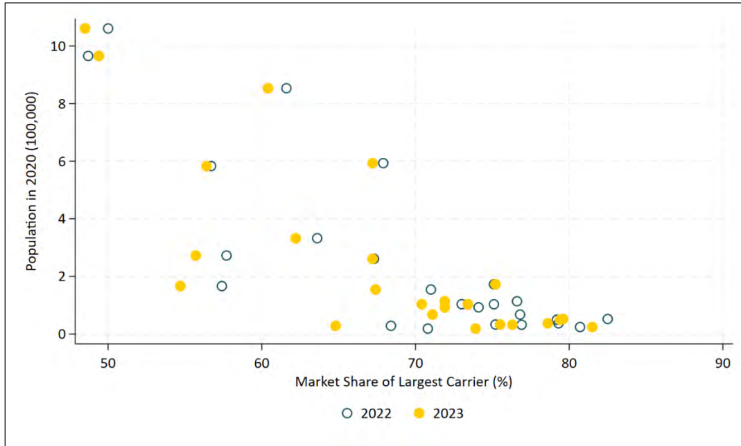
Figure 5. Relationship between County Size and Market Share of Largest Carrier, 2022 and 2023
